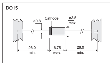
Package Dimensions (mm)
