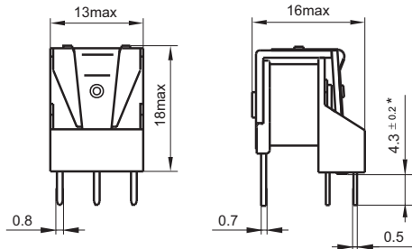
HFKM Unenclosed
