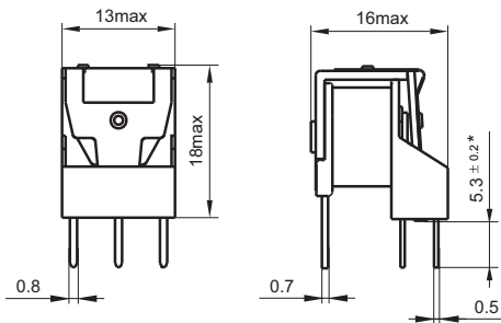
HFKS Unenclosed
