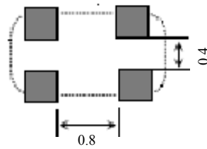
Pad Layout
