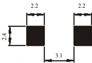
Pad layout
